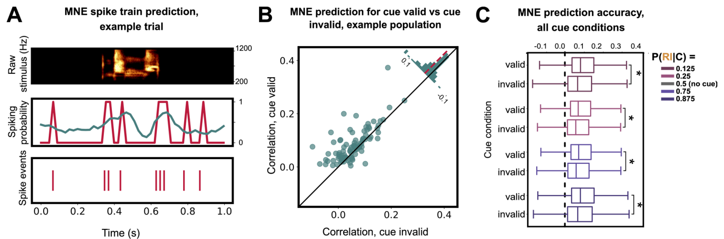
Extended Data Fig. 4 | Maximum Noise Entropy encoder model fit to neural data. (A) A sample MNE receptive field prediction. (top) Raw spectrogram of the target syllable on an individual trial. (middle) Actual (red) and receptive field model predicted (teal) spiking probability (same trial). (bottom) Raster plot of spiking events (same trial). (B) Correlation values between actual and predicted spiking for cue-valid vs. cue-invalid trials. Trial correlation values were averaged
